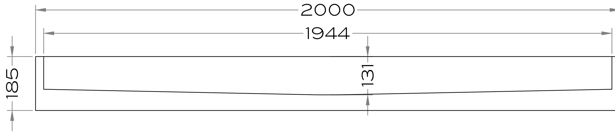
FRONT VIEW
