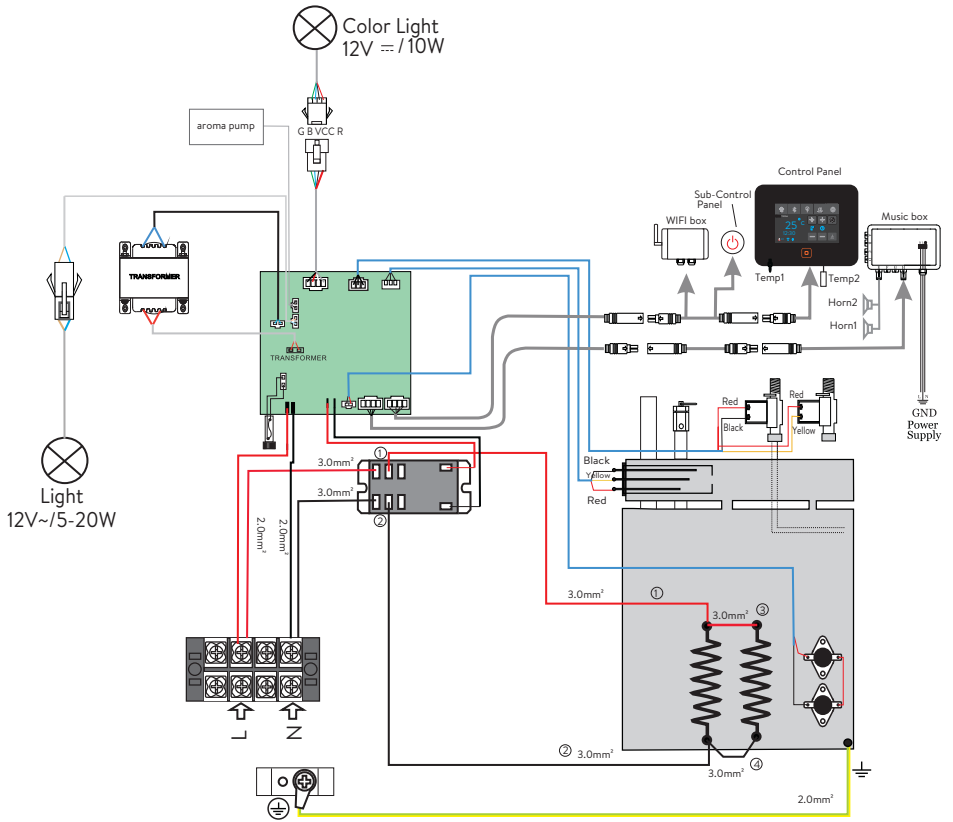
Figure(Heating element and Power line assemble illustration)
