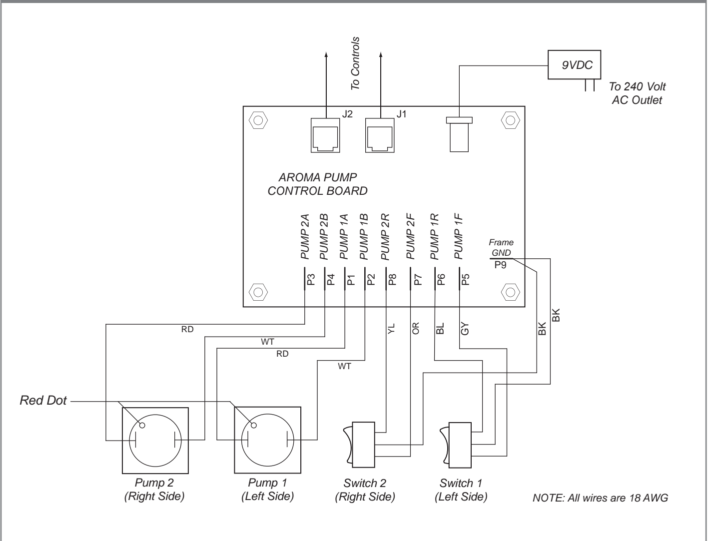
Figure 8: Wiring Diagram
