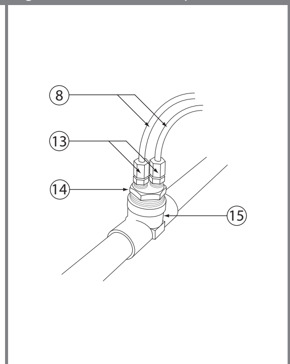
Figure 2: AromaSense Adapter
