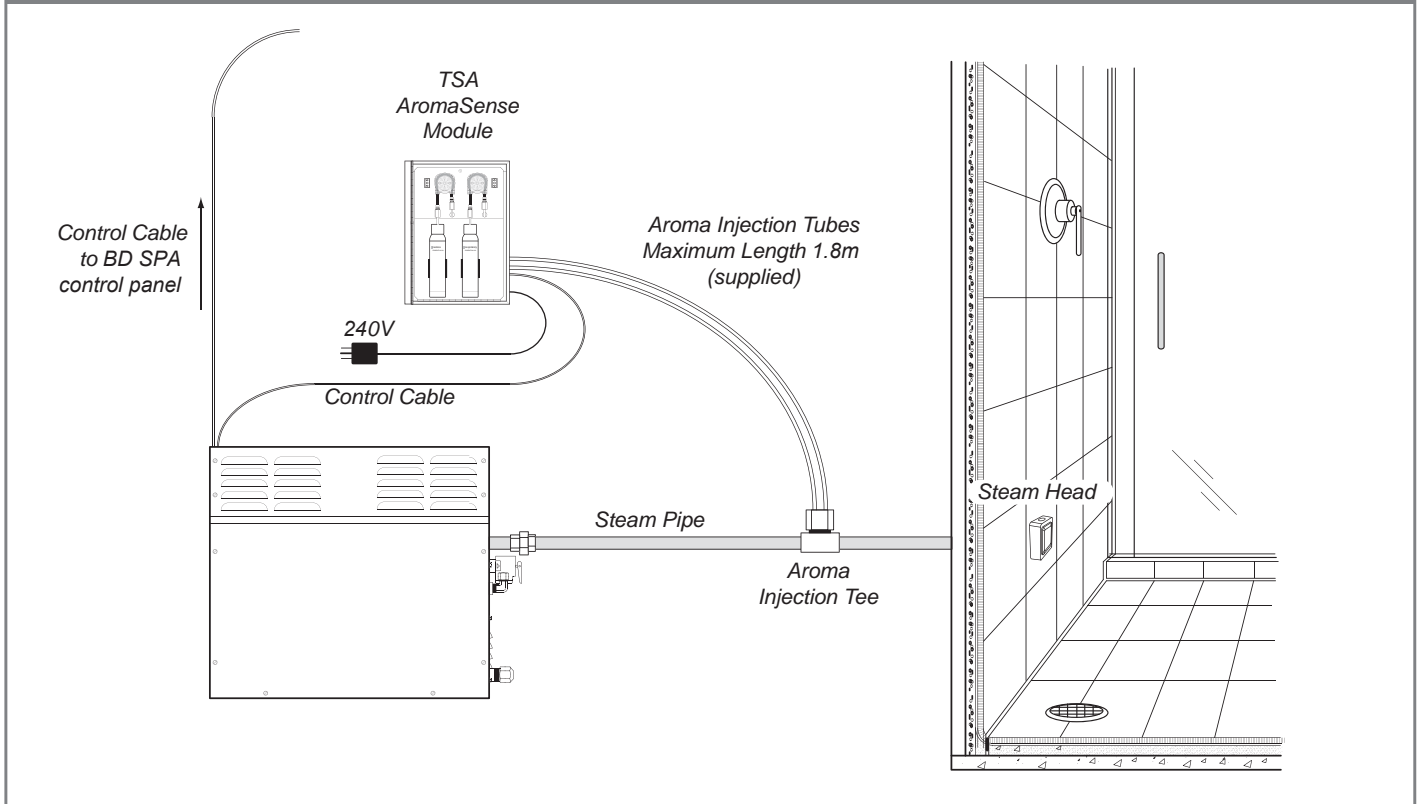
Figure 3 - Installation
