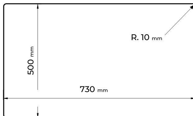
Counter top Cut-out template
