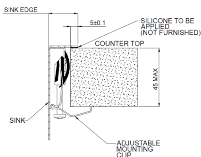
FASTENING DETAIL
