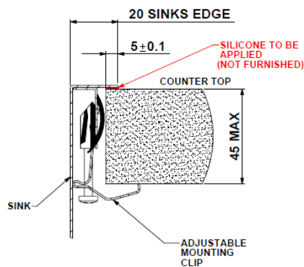
Fastening detail
