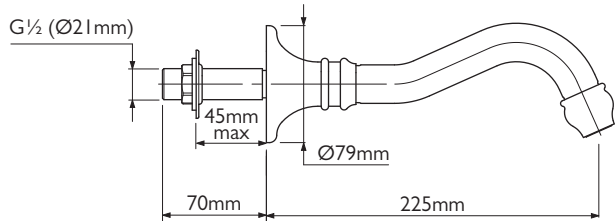
MK 2210 – Mackintosh bath wall spout
