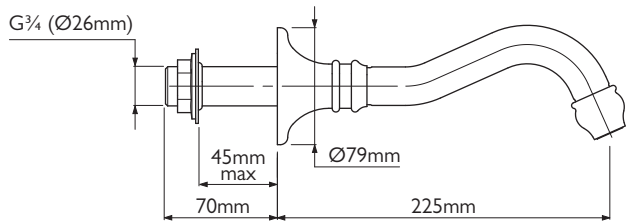
FRE 2210 – La Chapelle bath wall spout
